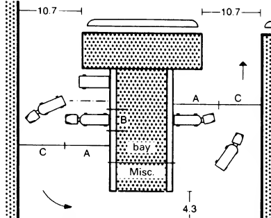
10 Loading and unloading in a courtyard
